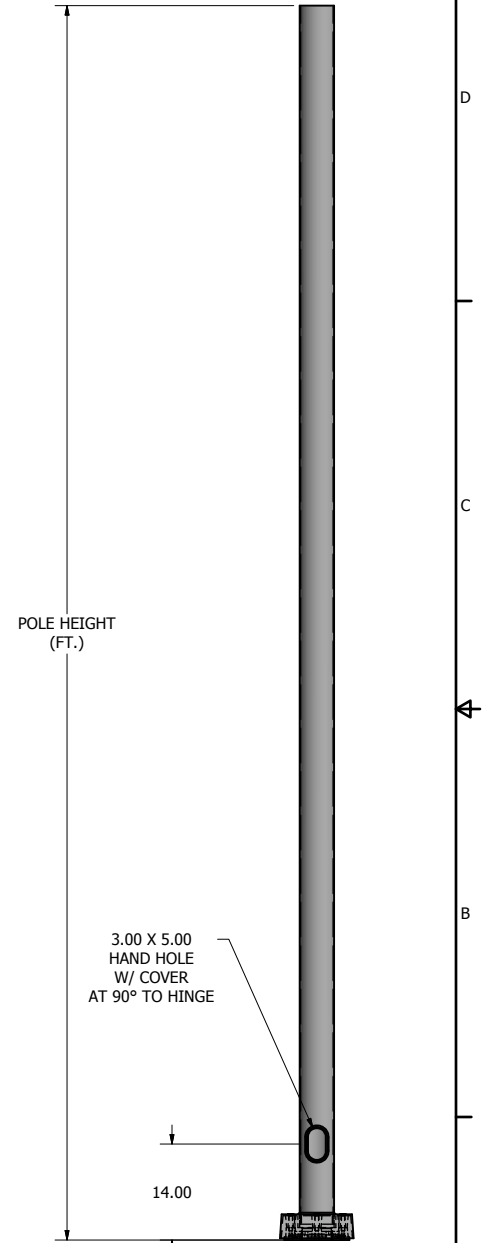
POLE DETAIL
